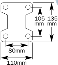
Top Plate - Wheel Dia. 200mm
