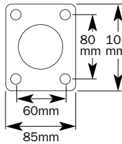
Top Plate - Wheel Dia. 80-125mm
